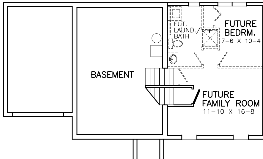
LOWER LEVEL PLAN 432 SQ.FT.
